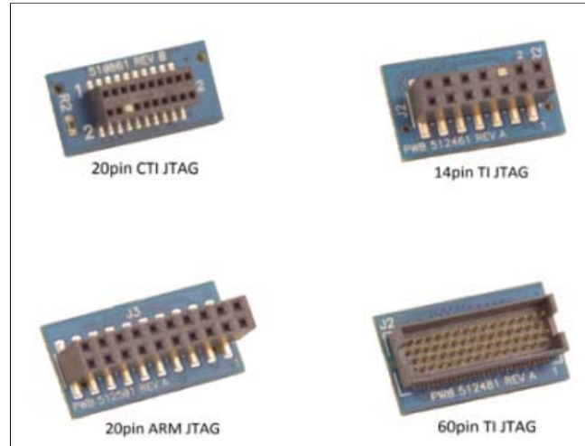
JTAG Cable Adapter kit for XDS560v2 STM
