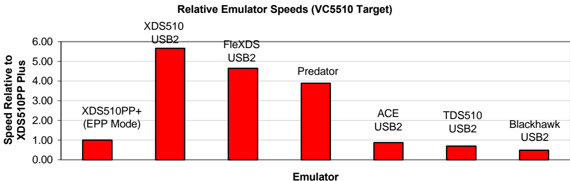
Figure 4: Relative Portable Emulator Speeds
