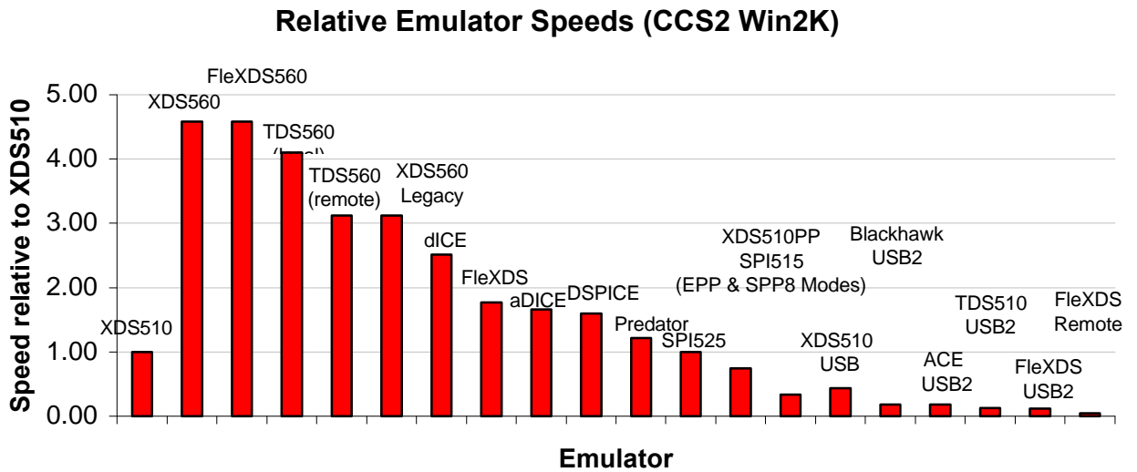
Figure 3: Relative Emulator Speeds
