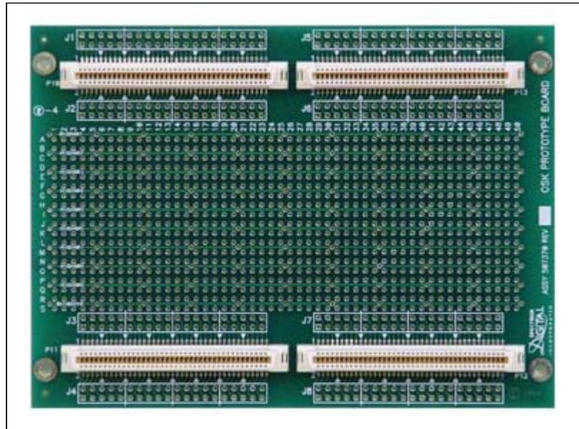
Wire Wrap Prototyping Module for OSKs
